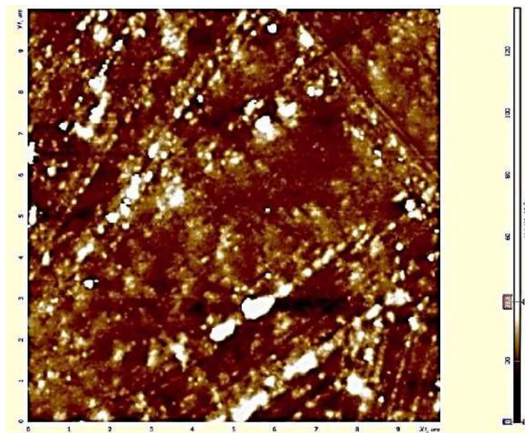
Fig.1. 2D image of the surface of Au- Ga 2 O 3 -n-GaP 0.4 As 0.6 nanostructures obtained by AFM. Sample №3
