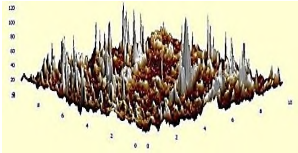
Fig 2. Three – dimensional image of the surface of Au- Ga 2 O 3 -n-GaP 0.4 As 0.6 nanostructures obtained by AFM. Sample №3
